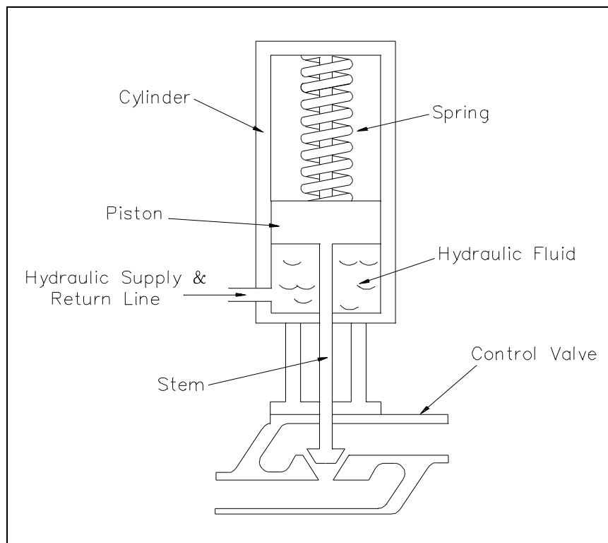
Figure 37 Hydraulic Actuator
