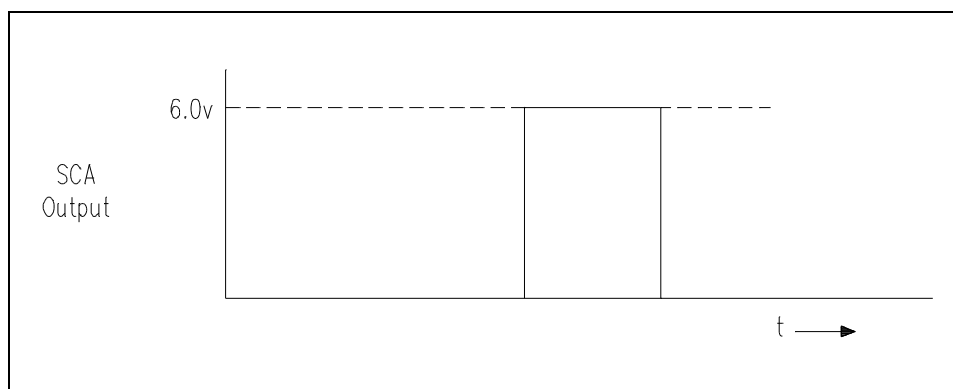
Figure 11 Single Channel Analyzer Output
