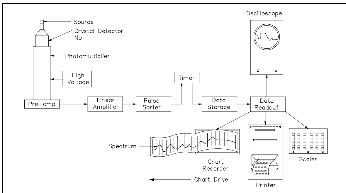
Figure 27 Gamma Spectrometer Block Diagram
