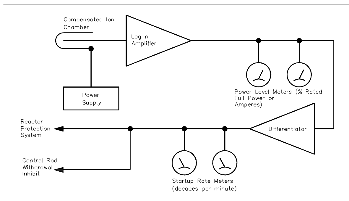
Figure 36 Intermediate Range Channel
