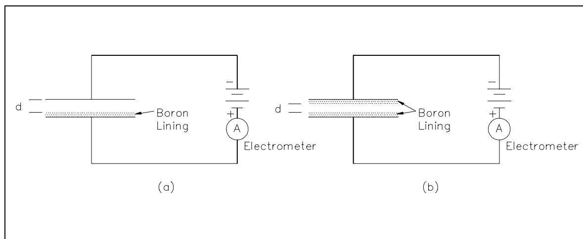
Figure 18 Minimizing Gamma Influence with Boron Coating Area
