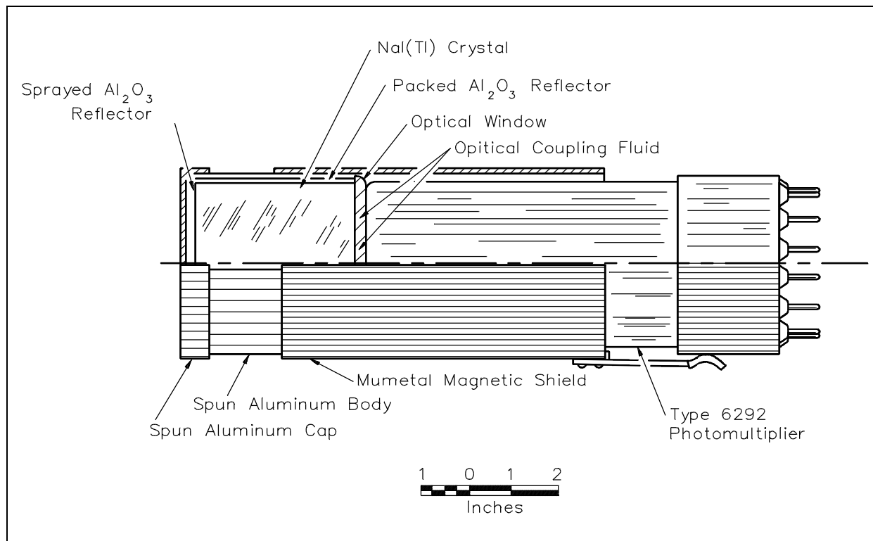
Figure 25 Scintillation Counter
