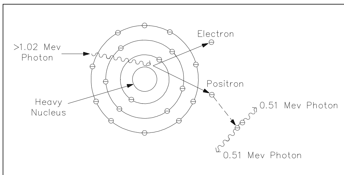
Figure 4 Pair Production
