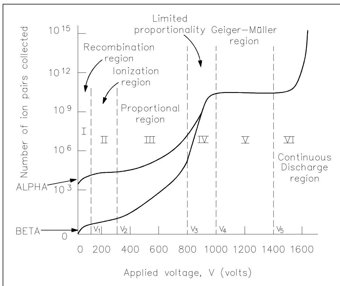
Figure 6 Ion Pairs Collected -vs- Applied Voltage
