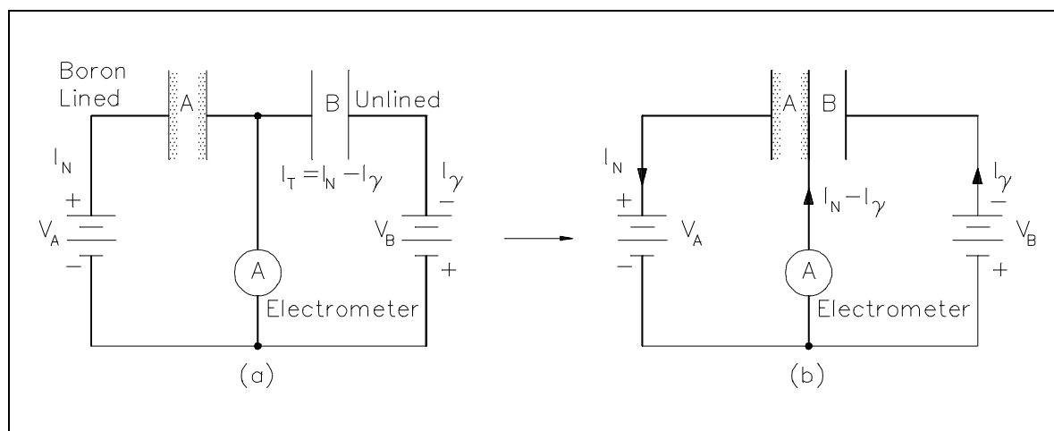
Figure 19 Compensated Ion Chamber
